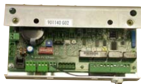
3215.15.7400 ECO board Quadro ECO
